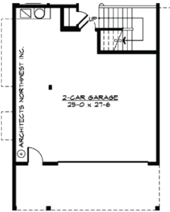
LOWER FLOOR PLAN
